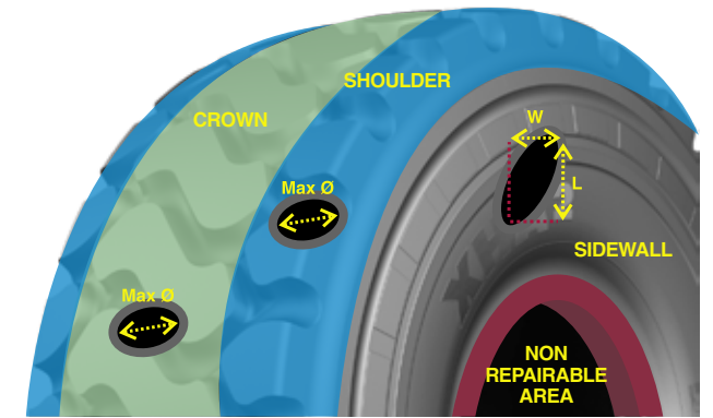
RADIAL/OTR NON-REPAIRABLE AREA
